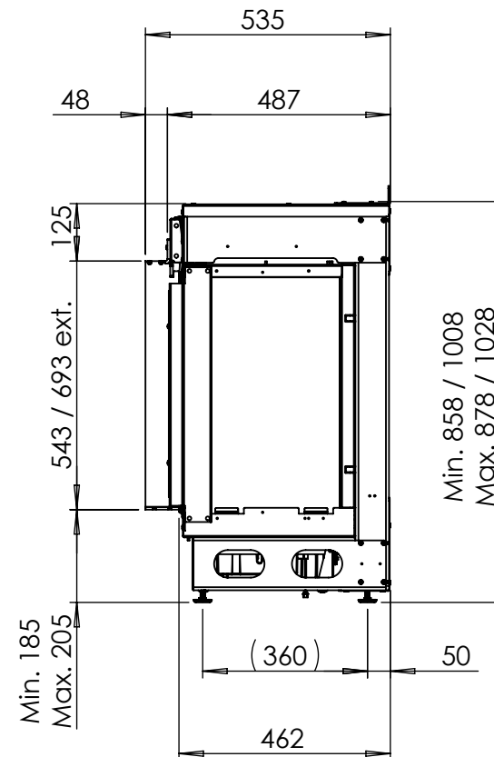
Dimensional Drawing e-MatriX Mood 800/500 I + e-MatriX Mood 800/650 I
